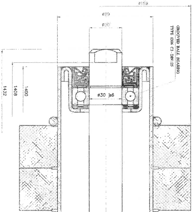
DETAIL Y SCALE FULL
